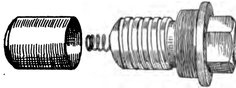
FIG. 72.—Air discharge valve.
